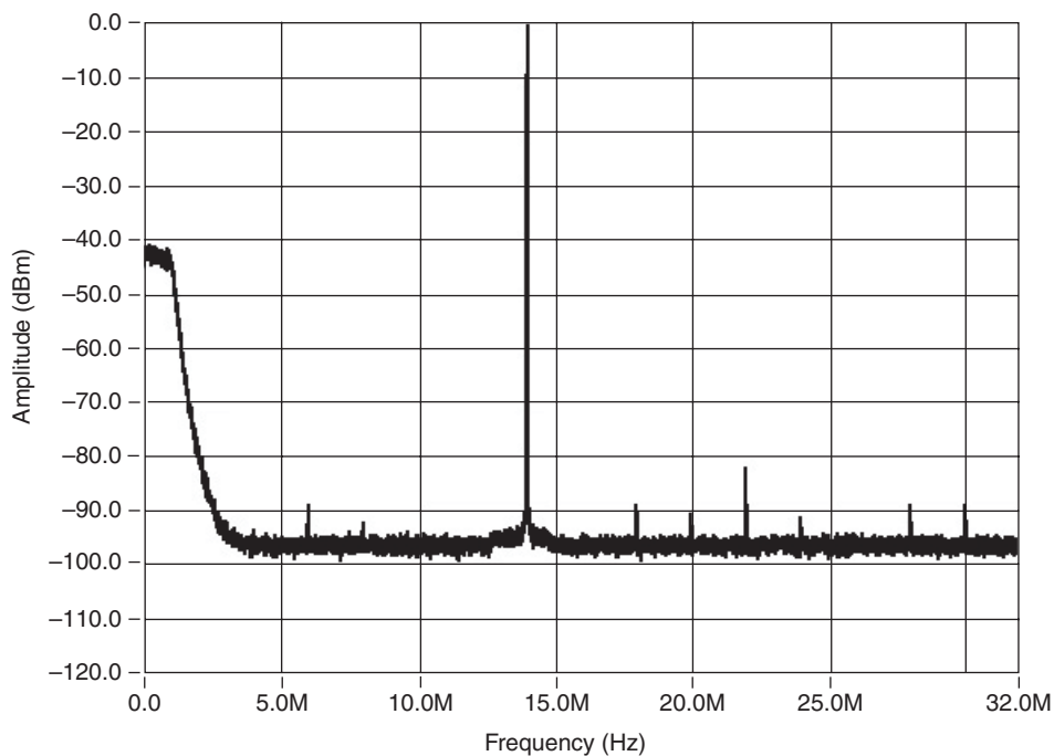
Figure 2. Harmonic Distortion (14 MHz at 0 dBm)
