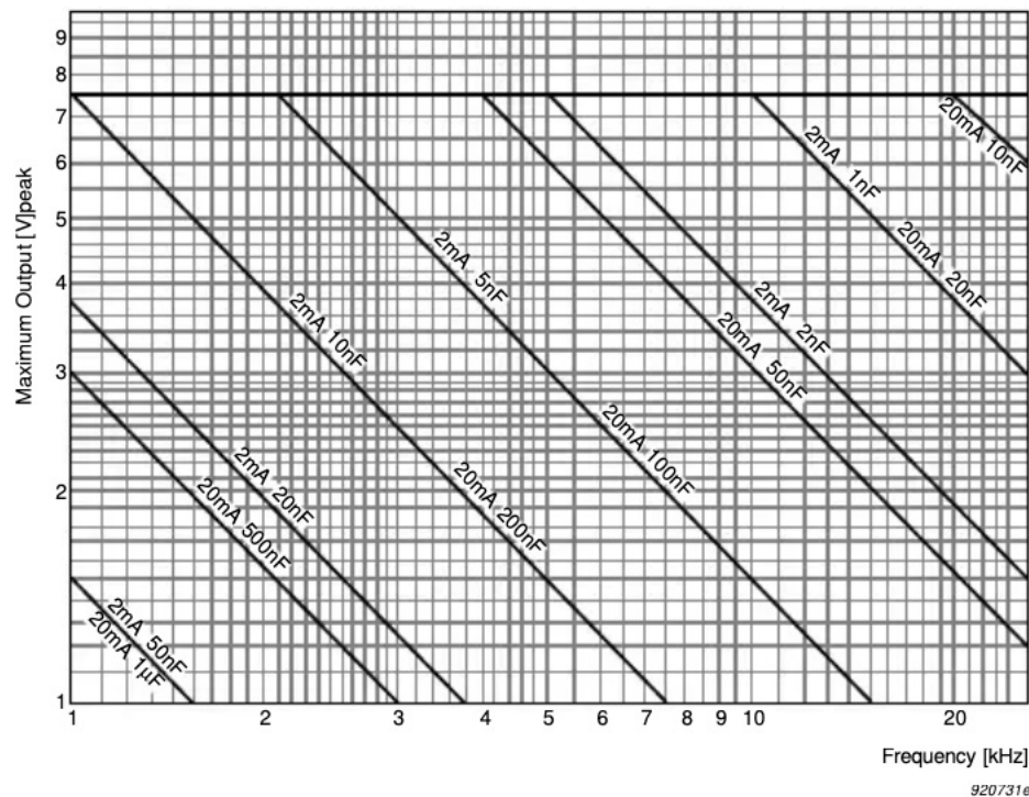
Fig. 6 Typical curves for maximum output level of DeltaTron® accelerometers, showing maximum capacitive load over the recommended current supply range
