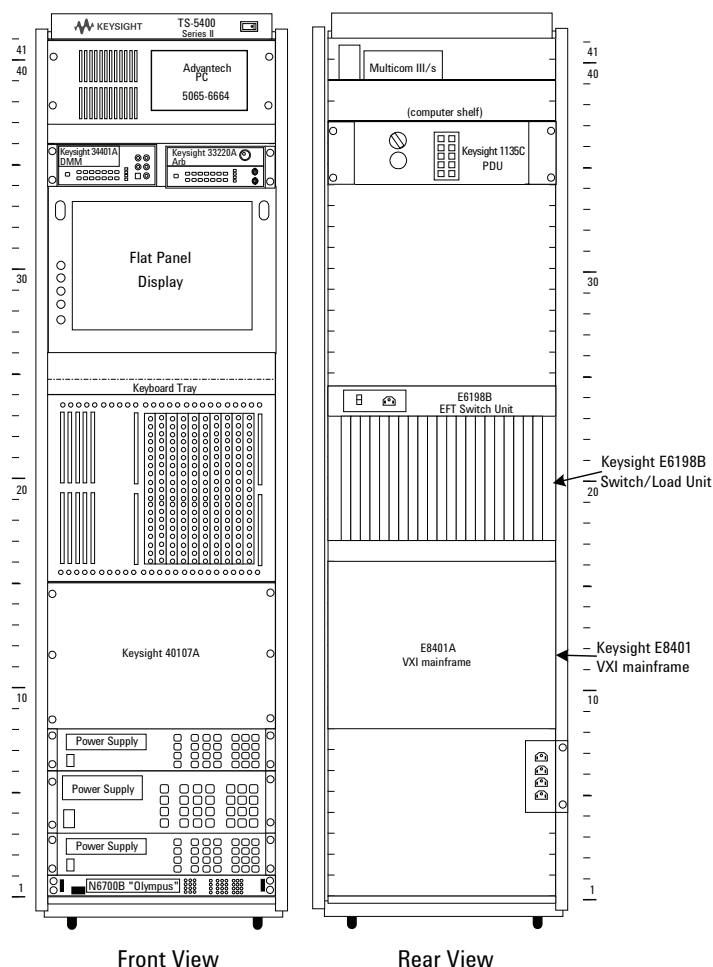
Figure 4. VXI/GPIB Express Connect (front and rear views)
