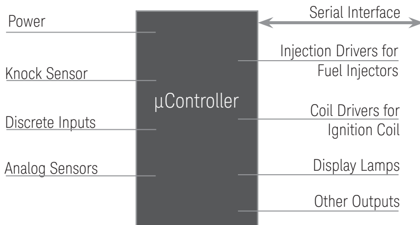
Figure 7. Serial interface for engine control ECM
