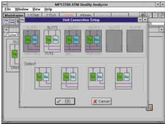
Setting signal path for different units
