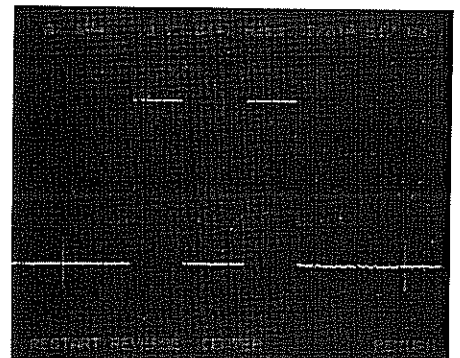
The RESTART feature at work: Place the cursors over the area of interest, touch "RESTART" and the PM 3350 automatically calculates proper delay, and time base settings to capture any signal detail that has been selected by the user.
